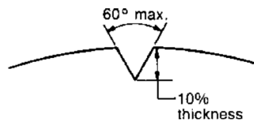
FIGURE C1 N10 NOTCH
