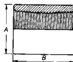
(b) Series RC internal taper pipe thread to AS 1722.1 available when specified (see Clause 3.4)
