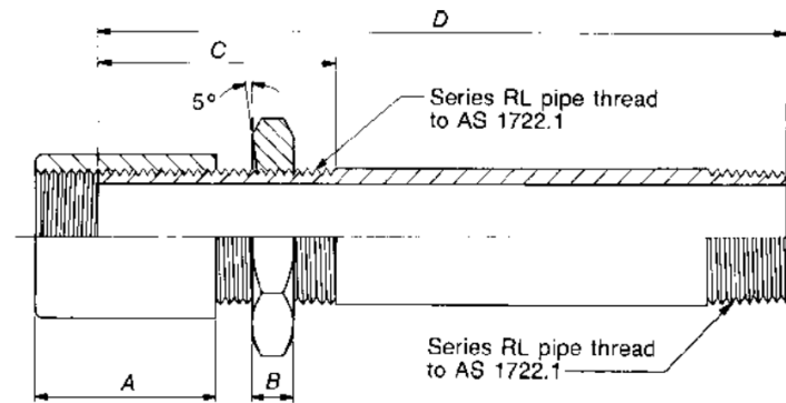
(a) Single longscREW
