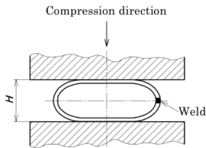
Figure 2 Flattening test (ring test piece)
