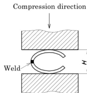
Figure 3 Flattening test (C-shaped test piece)
