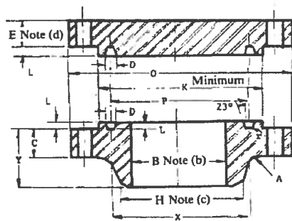
RING-TYPE JOINT
