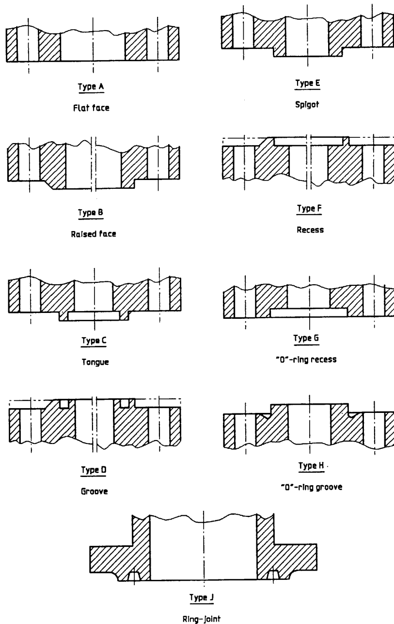
Figure 5 — Illustration of flange facings (types A to J)
