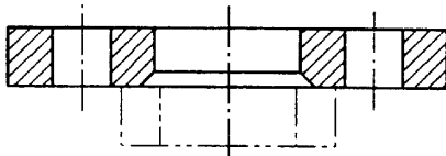
Type 02 Loose plate flange with weld-on plate collar (see type 32)
