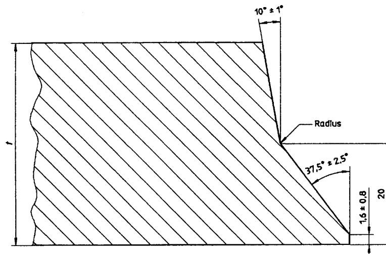
b) t greater than 22 mm (pipeline applications)
