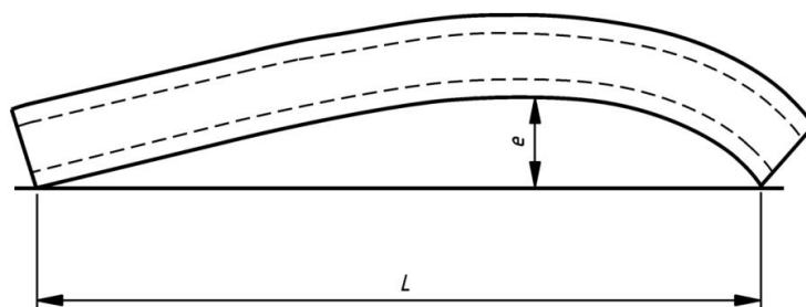
Figure 8 — Measurement of deviation from straightness
