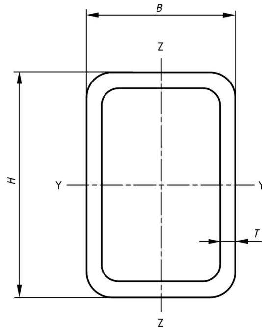
Figure B.3 — Rectangular hollow section
