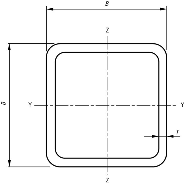
Figure B.2 — Square hollow section
