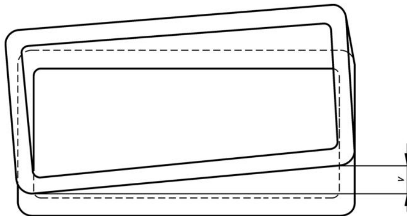
Figure 5 — Twist of square or rectangular hollow sections
