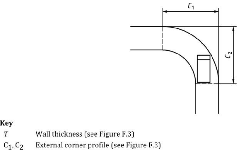
Figure F.4 — Location of test pieces (subsized) for the impact test for square and rectangular hollow sections in the corner region
