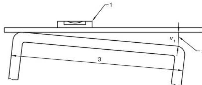
FIGURE 5 TOTAL TWIST OF SQUARE OR RECTANGULAR HOLLOW SECTIONS
