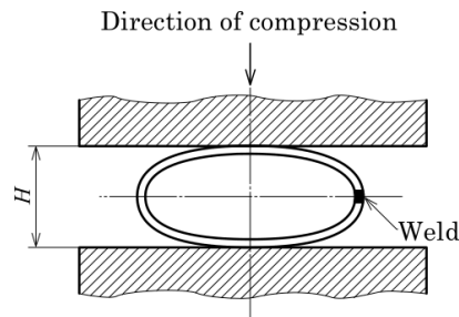
Figure 2 Flattening test
