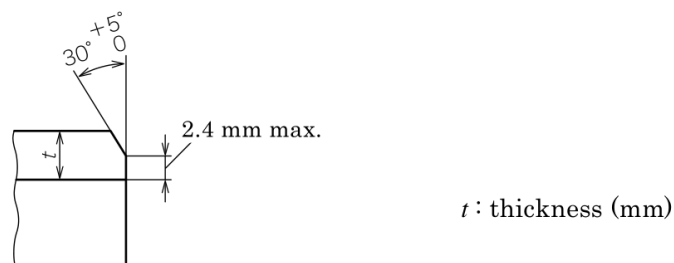
Figure 1 Shape of bevel end
