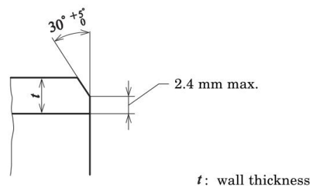
Figure 1 Shape of bevelled end
