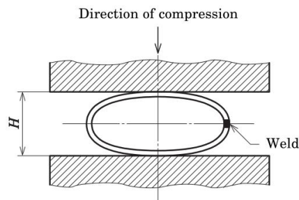
Figure 2 Flattening test
