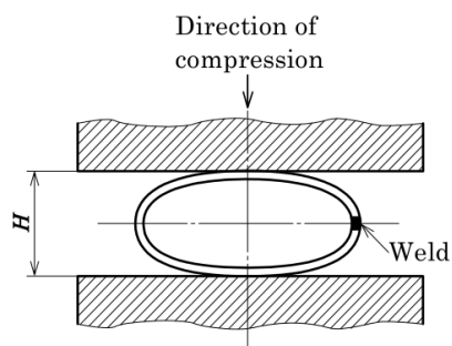
Figure 2 Flattening test (ring test piece)
