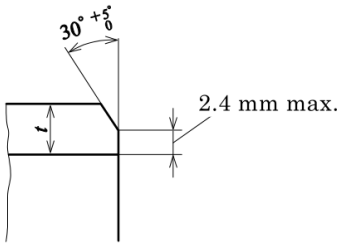
Figure 1 Shape of bevelled end
