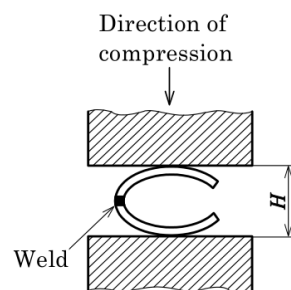
Figure 3 Flattening test (C-shaped test piece)
