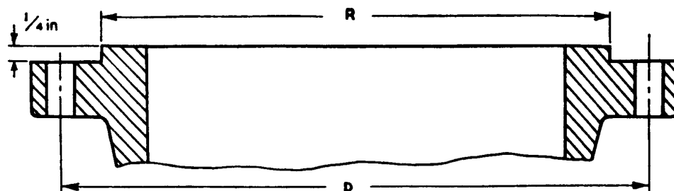
Raised face type—welding-neck and slip-on
