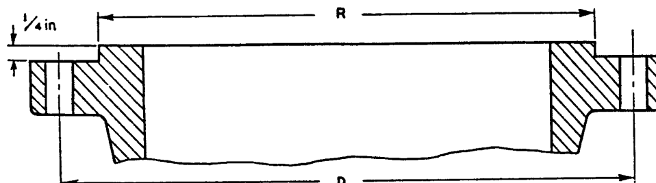
Raised face type—welding-neck and slip-on
