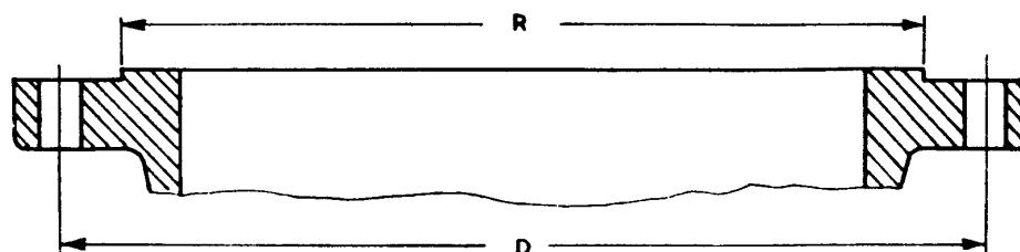
Raised face type—welding-neck and slip-on
