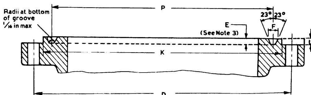
Ring-joint type—welding-neck and slip-on
