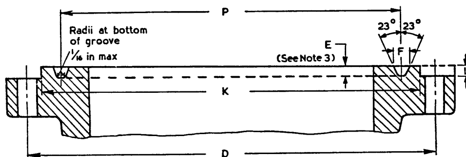
Ring-joint type—welding-neck and slip-on
