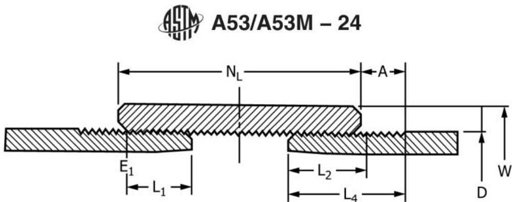
FIG. X3.2 Dimensions of Hand Tight Assembly for Use with Table X3.2
