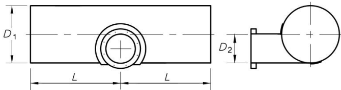
FIGURE D12 TANGENTIAL DRAIN OR SCOUR OUTLET
