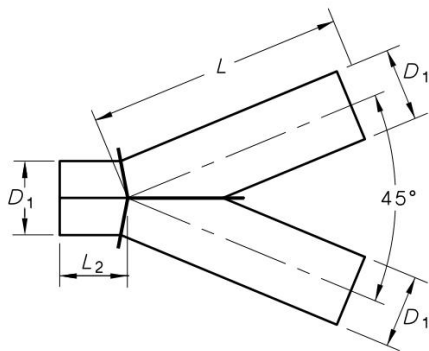
FIGURE D9 Y-PIECE
