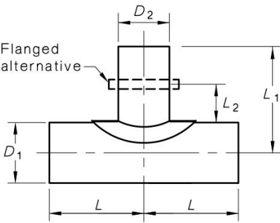
FIGURE D6 UNEQUAL TEE WITH REINFORCEMENT COLLAR
