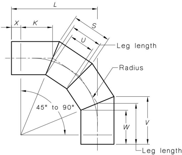
FIGURE D3 MITRED BEND 45° TO 90°
