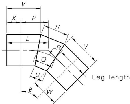
FIGURE D2 MITRED BEND 22.5° TO 45°
