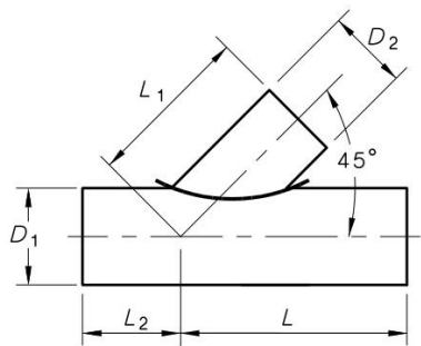
FIGURE D7 REINFORCED BRANCH
