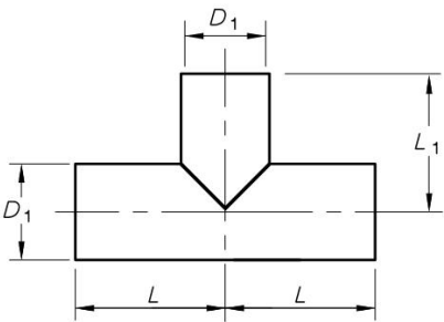
FIGURE D4 EQUAL TEE (UNREINFORCED)
