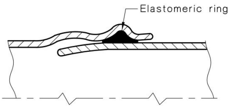
FIGURE E2 ELASTOMERIC RING JOINT
