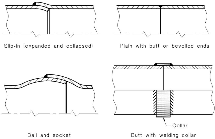
FIGURE E1 WELDED JOINTS
