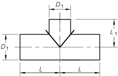
FIGURE D5 REINFORCED EQUAL TEE
