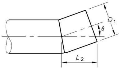
FIGURE D14 PIPE SUPPLIED WITH ANGLE DEVIATION
