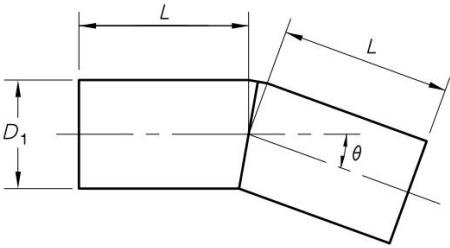
FIGURE D1 MITRED BEND 0° TO 22.5°
