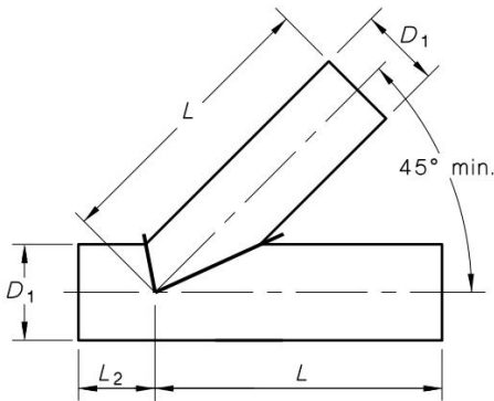
FIGURE D8 REINFORCED ANGLE BRANCH
