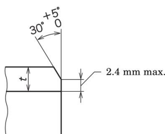
Figure 1 Shape of bevel end
