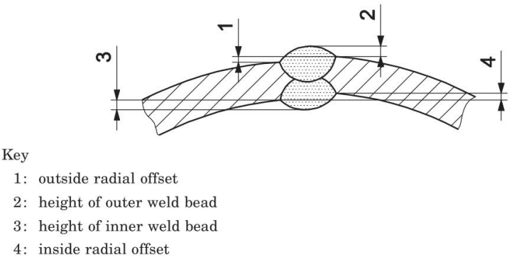
Figure 2 Weld bead height with radial offset
