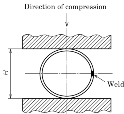
Figure 1 Flattening test (using ring-shaped test piece)
