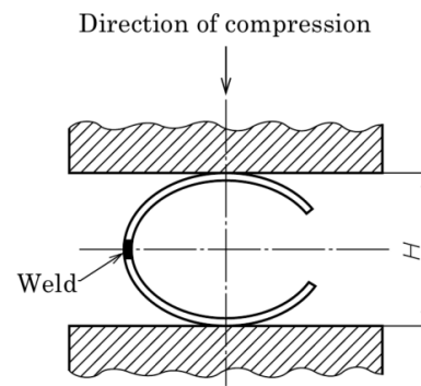
Figure 2 Flattening test (using C-shaped test piece)
