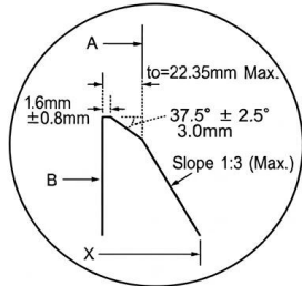
BEVEL FOR WALL THICKNESS(to) 0.88" IN.(22.35mm) OR LESS.
