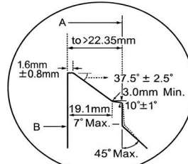
BEVEL FOR WALL THICKNESS(to) GREATER THAN 0.88 IN.(22.35mm)
