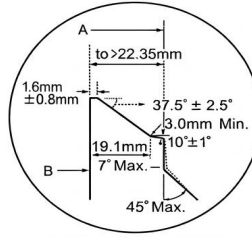
BEVEL FOR WALL THICKNESS( t ) GREATER THAN 0.88 IN.(22.35mm)
